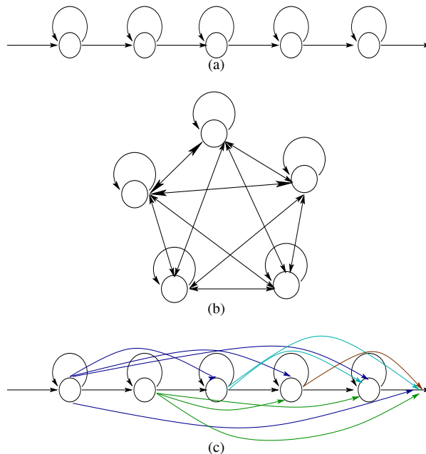
Fig. 1. (a) Mod0: Traditional 5-state sequential phone model (b) Mod1: Fully connected states inside a phone model (c) Mod2: Forward connected states inside a phone model. Note that in Mod1 and Mod2, any state could be a beginning state or an ending state.
