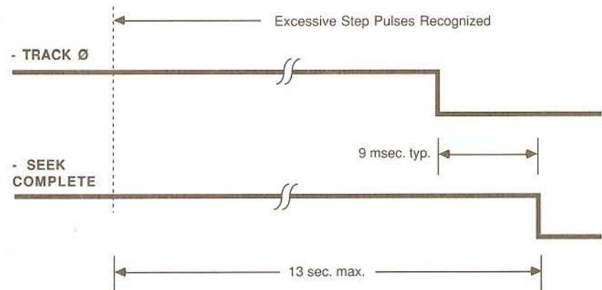
FIGURE 6: Auto-Truncation Timing
