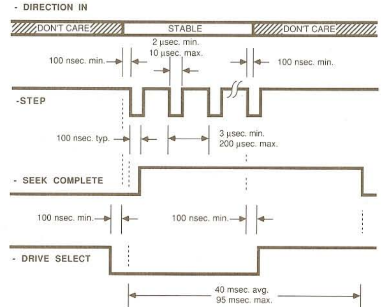
FIGURE 5: Buffered-Seek Timing
