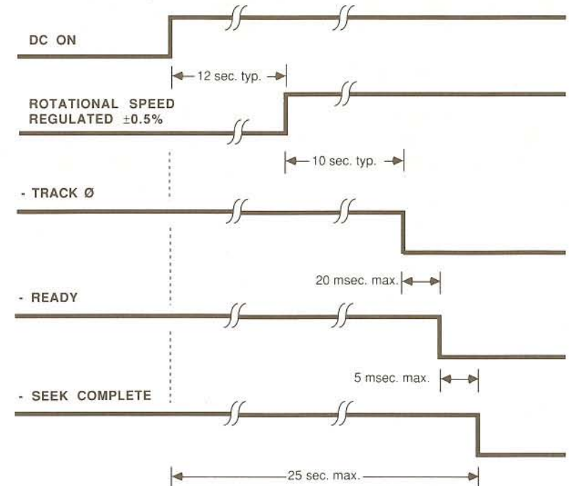
FIGURE 2: Typical Power-On Sequence
