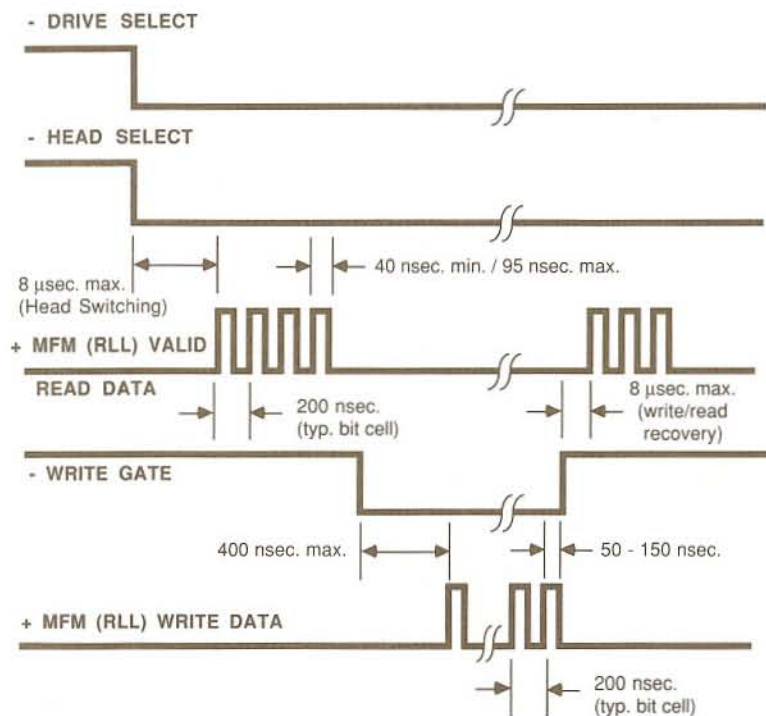
FIGURE 4: Read/Write Timing
