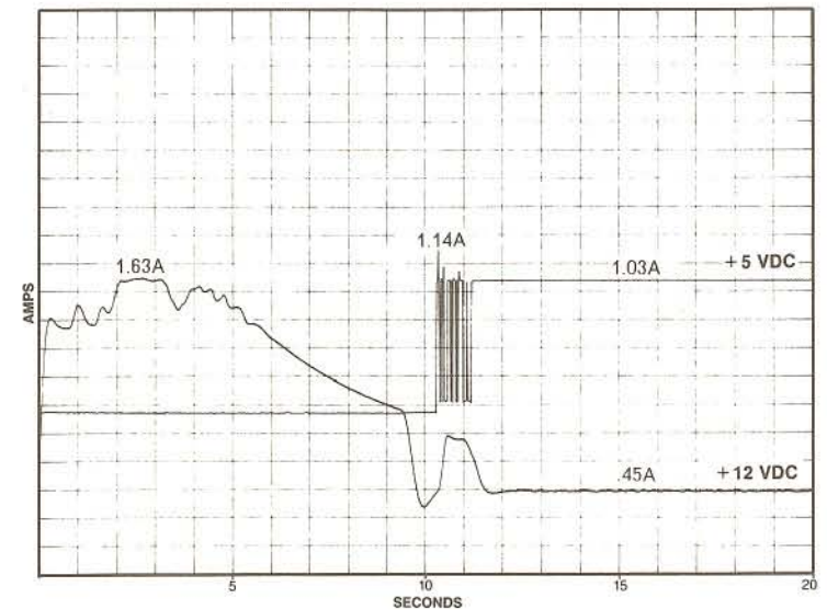
FIGURE 1: Typical +12 VDC Start-Up Current Profile
