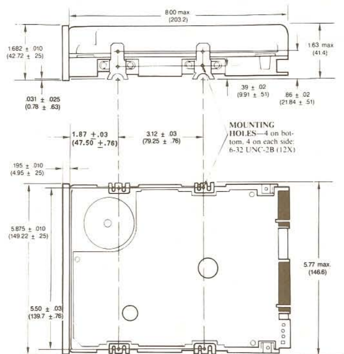
FIGURE 3: Drive Mounting Dimensions
